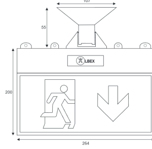
SURFACE MOUNTED
